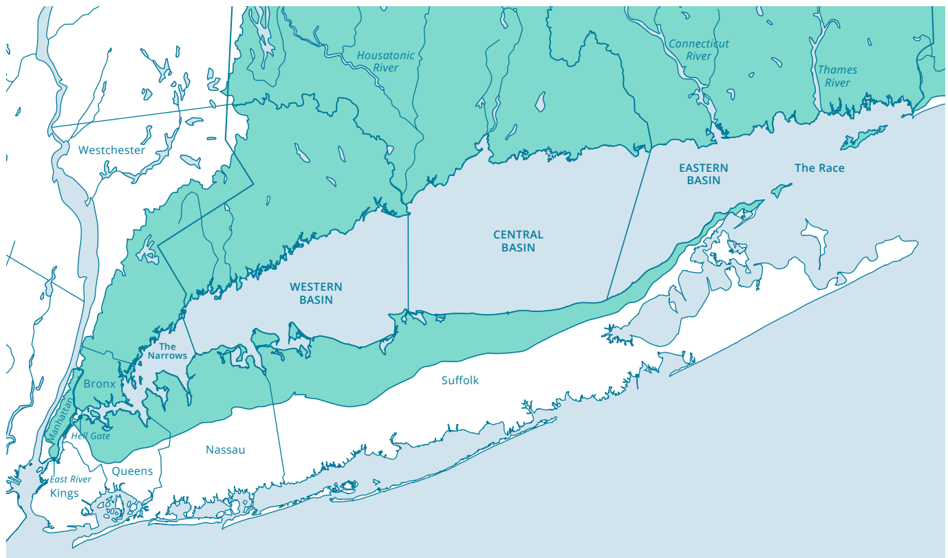
FIGURE 1. Long Island Sound and its basins and channels.
